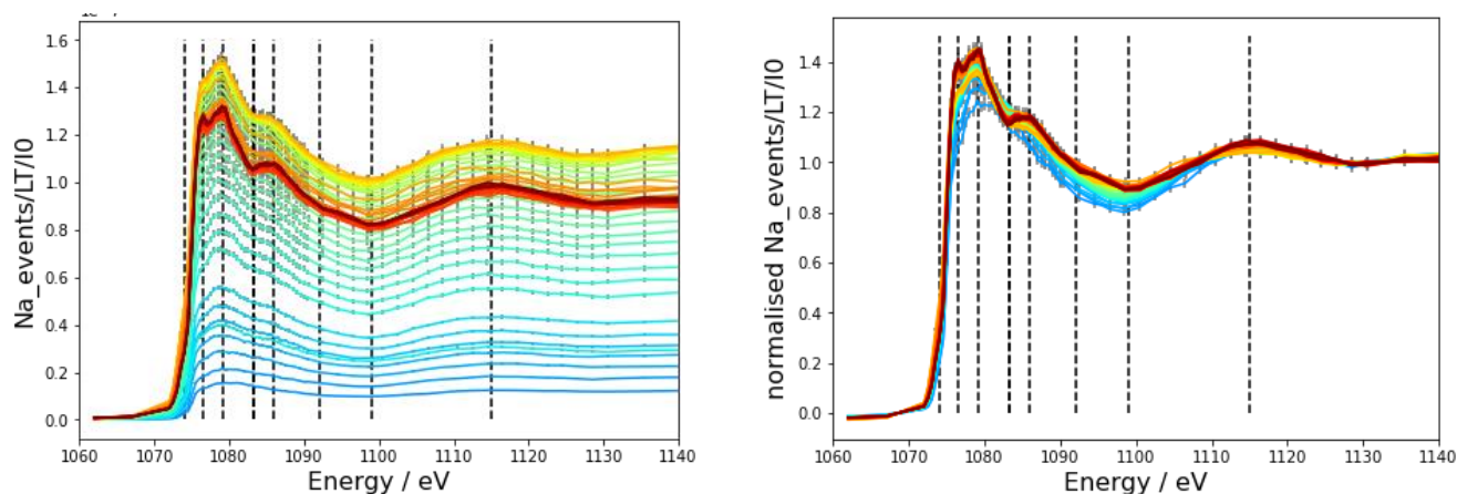
Figure 1 Operando XANES measurements at Na K-edge of HC composed electrode, a not normalized and b normalized ones.
